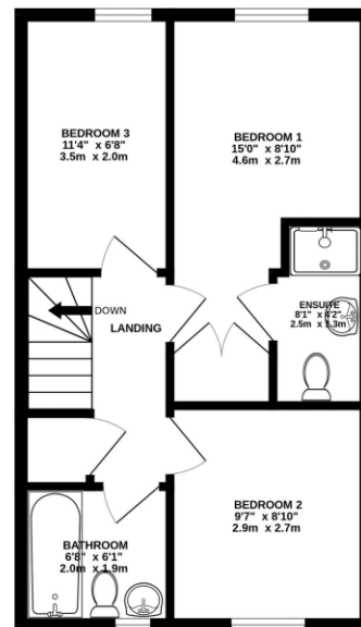
1ST FLOOR 413 sq.ft. (38.4 sq.m.) approx.
